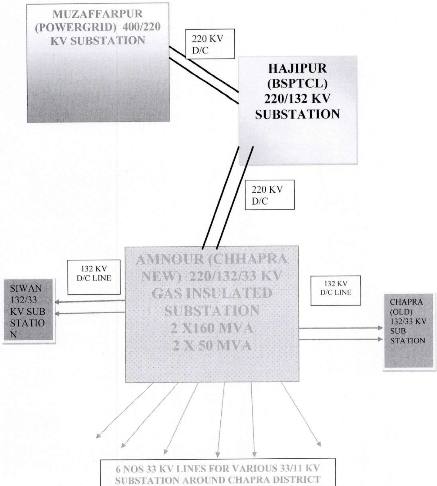
Figure 1: The present connectivity of Amnour Sub-station is represented below:
